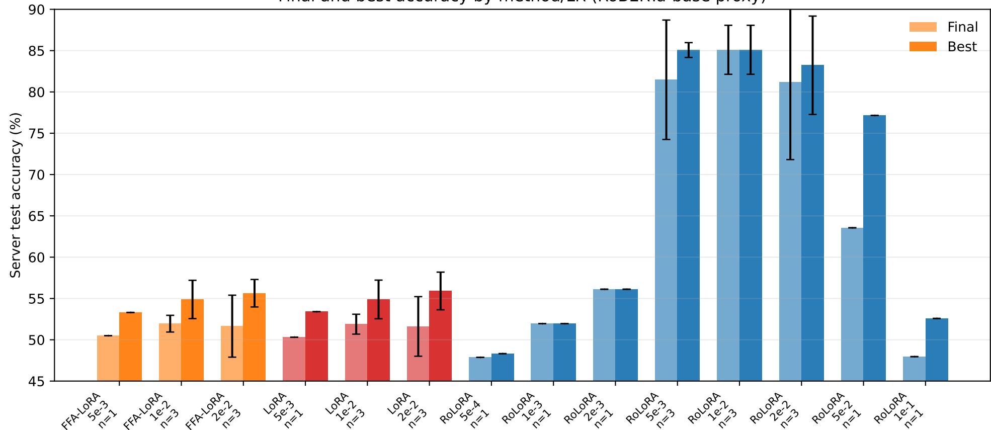
Final and best accuracy by method/LR (RoBERTa-base proxy)
