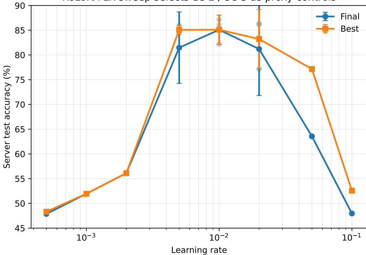
RoLoRA LR sweep selects 1e-2 / 5e-3 as proxy controls
