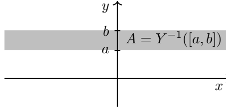
Figure 3.5: Conditional expectation w.r.t. \sigma(Y) : Horizontal strips A = Y^{-1}([a, b]) = \{\omega = (x, y) : a \leq y \leq b\} generate \sigma(Y) and are the typical elements in \sigma(Y) . The conditional expectation of X w.r.t. Y corresponds to averaging X w.r.t. \mathbf{P} over such a thin horizontal strip.
