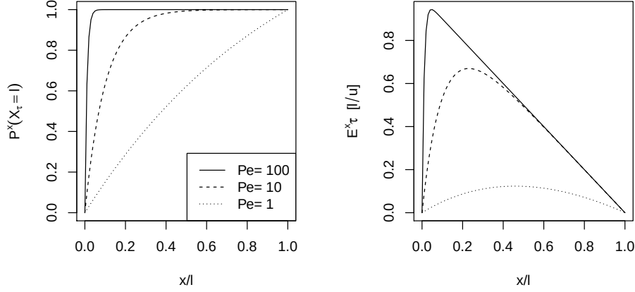
Figure 11.1: Exit behavior for Brownian motion with drift, for various Péclet numbers. Left panel: The probability of exiting to the right, as a function of the dimensionless initial position x/l . Right panel: The expected time to exit, as a function x/l , and measured in units of the advective time scale l/u .
