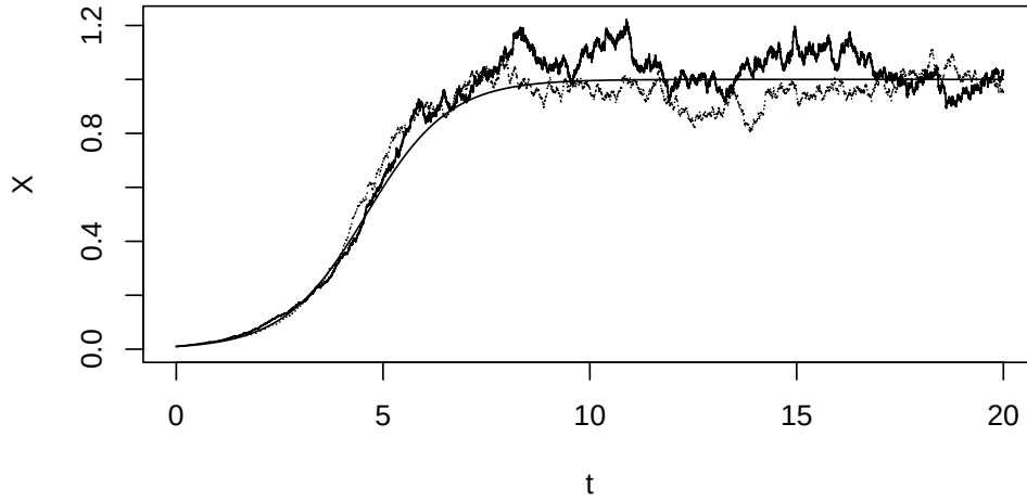
Figure 1.3: Two simulated sample paths (solid and dotted erratic curves) of the stochastic logistic growth model (1.5) with g(x) = \sigma x of a bacterial population with g(x) = \sigma x . A noise-free simulation is included (thin black line). Parameters are r = K = 1 , \sigma = 0.1 , X_0 = 0.01 . The computational time step used is 0.001.
