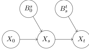
Figure 9.2: The Markov structure of solutions to stochastic differential equations. Here, B_0^s is shorthand for \{B_u : 0 \leq u \leq s\} while B_s^t is shorthand for \{B_u - B_s : s \leq u \leq t\} .
