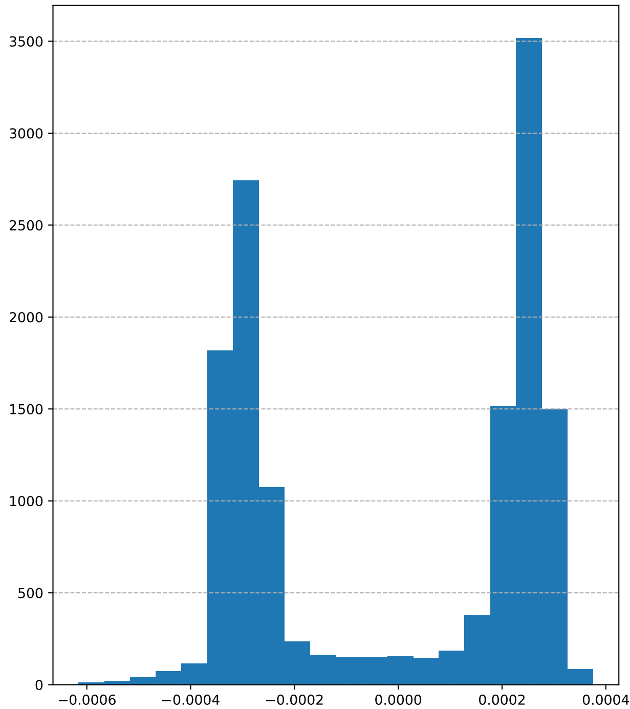
Distribution of variables for R_0
