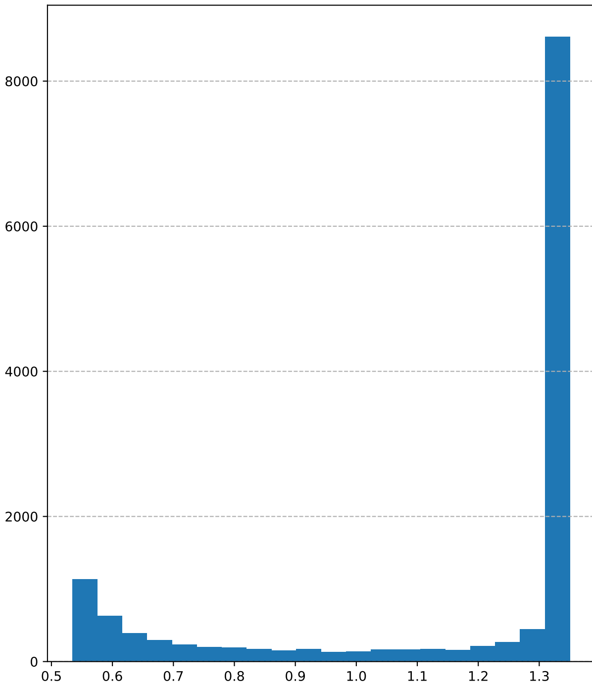
Distribution of variables for R_0
