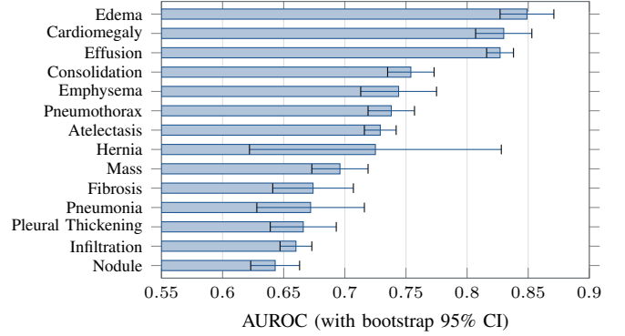
Fig. 5. Per-label test AUROC on ChestMNIST (DenseNet-121, 64 px source upsampled to 224 px, CPU, best of four epochs, N_{\text{test}}=12,000 ), with bootstrap 95% CI whiskers, sorted ascending. The ordering tracks how visible each finding is, and every interval clears the 0.5 chance line. Eleven of these labels nonetheless emit no positive prediction at the default threshold (Section V-B).
