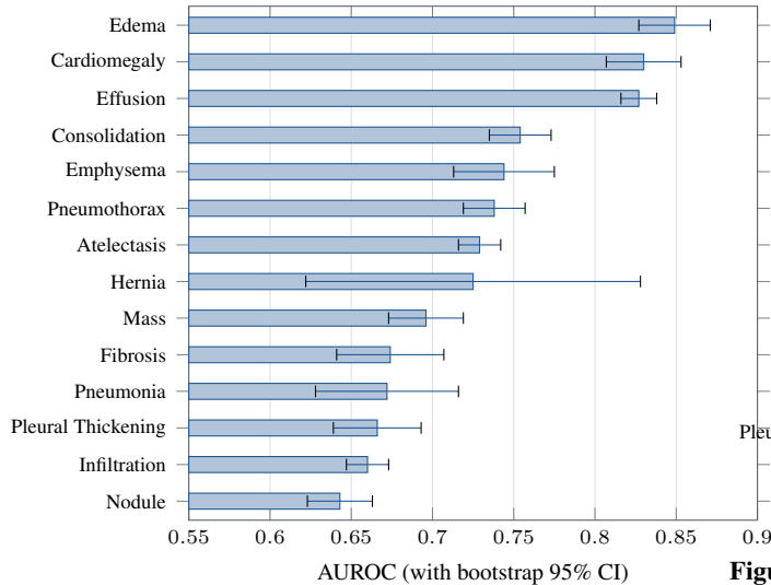
Figure 4: Measured per-label test AUROC on ChestMNIST (DenseNet-121, 64 px, CPU), with bootstrap 95% CI whiskers, sorted ascending. The ordering is clinically sensible: readily visible findings (Edema, Cardiomegaly, Effusion) top the chart, subtle small ones (Nodule, Infiltration) sit lowest, and every interval clears the 0.5 chance line, which indicates the model learned real structure.
