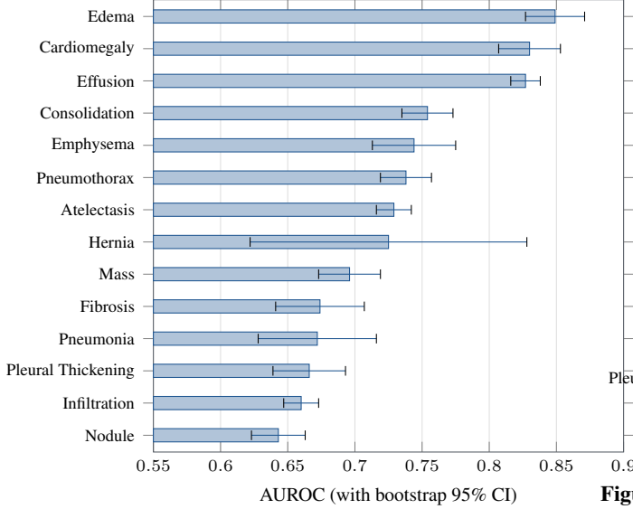
Figure 4: Measured per-label test AUROC on ChestMNIST (DenseNet-121, 64 px, CPU), with bootstrap 95% CI whiskers, sorted ascending. The ordering is clinically sensible: readily visible findings (Edema, Cardiomegaly, Effusion) top the chart, subtle small ones (Nodule, Infiltration) sit lowest, and every interval clears the 0.5 chance line, which indicates the model learned real structure.
