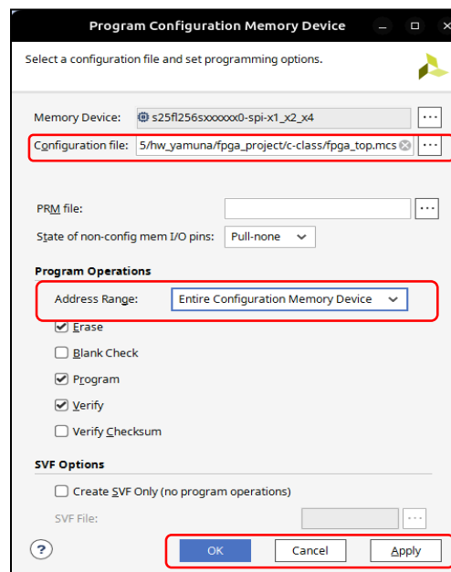
Figure 7.6: Program Configuration Memory Device
