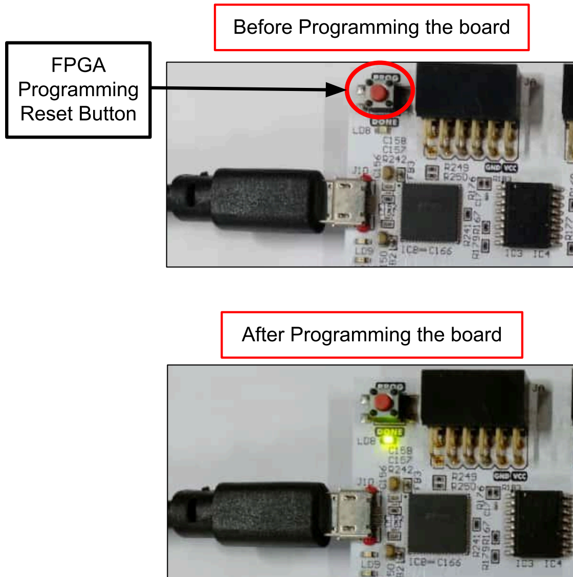
Figure 8.1: Before Programming vs After Programming
