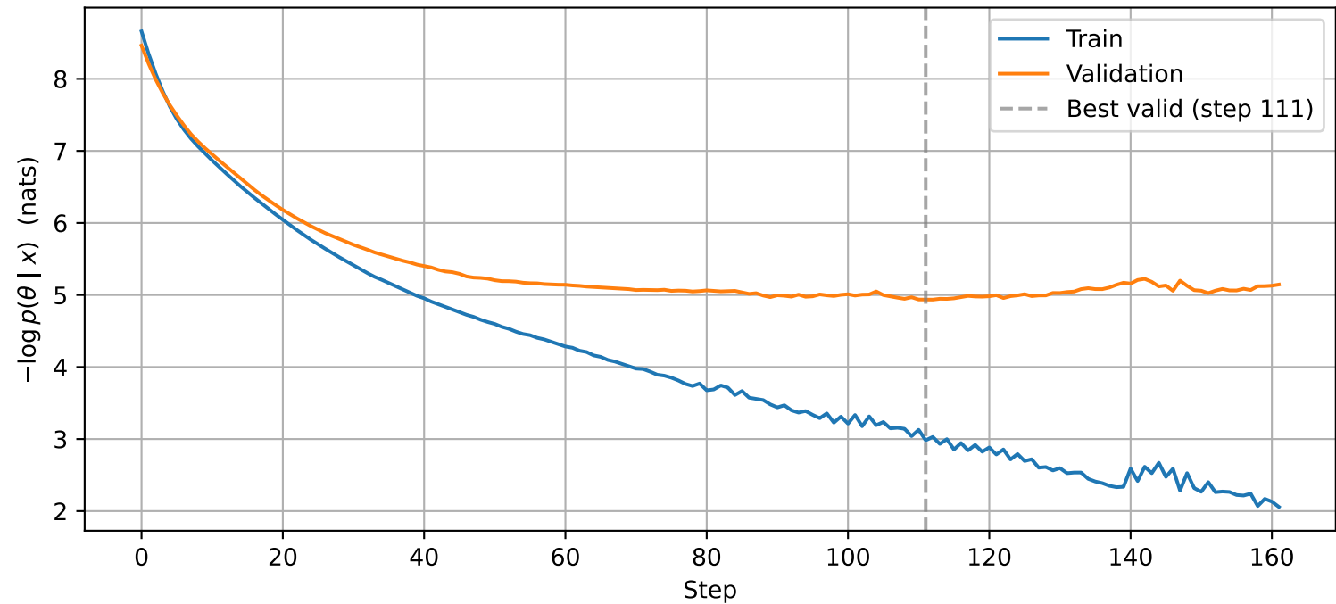
Loss Curve — combined
