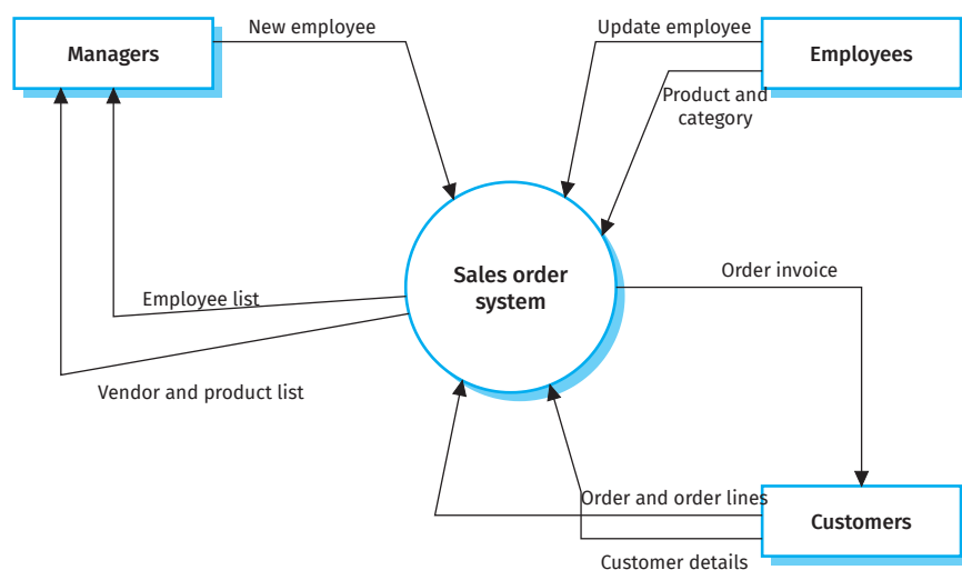
Figure 5.3 Context diagram (level-0 DFD) of a sales order system
