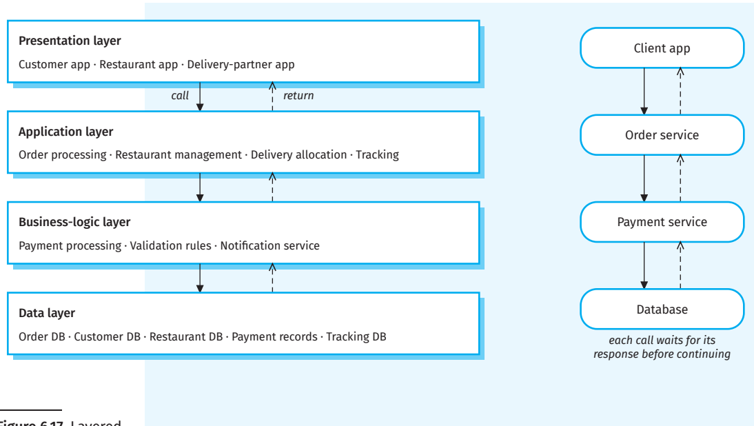
Figure 6.17 Layered architecture of a food-delivery system with call-and-return control
