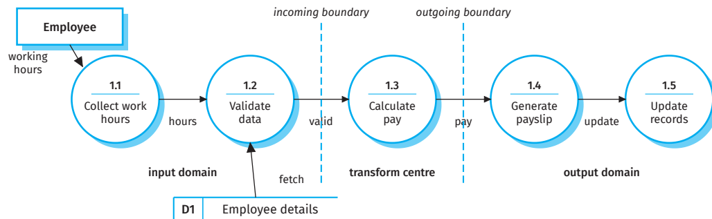
Figure 6.22 Payroll DFD with its flow boundaries
