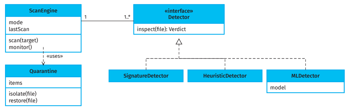
Figure 5.28 Class-based element: principal classes of the antivirus product
