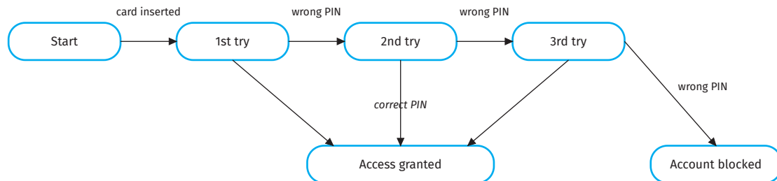
Figure 8.18 State transition diagram for PIN entry at an ATM
