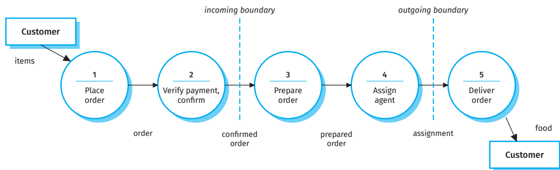
Figure 6.21 DFD of the food-delivery workflow
