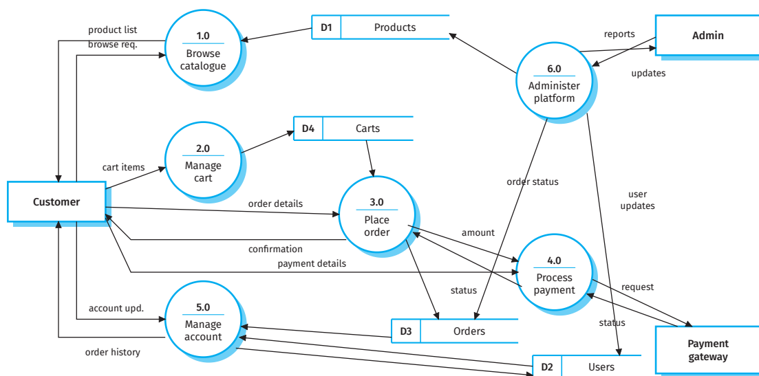
Figure 6.28 Level-1 DFD of the online shopping system
