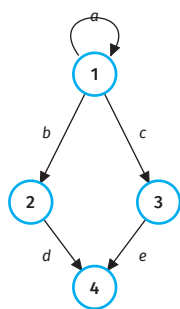
Figure 8.14 A flow graph with a self-loop, and its graph and connection matrices
