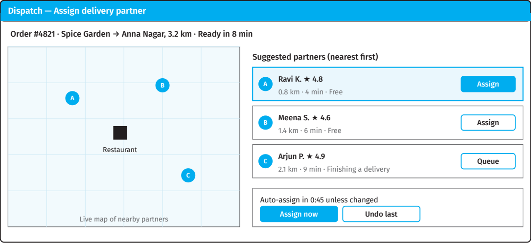
Figure 7.11 Layout of the delivery partner assignment screen
