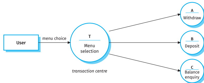
Figure 6.25 ATM DFD showing transaction flow
