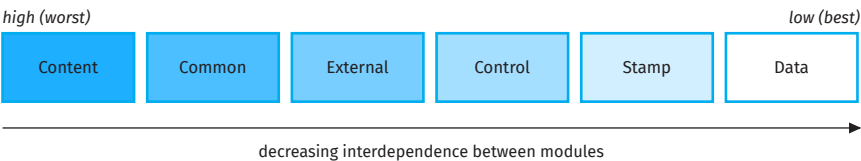
Figure 7.6 The scale of coupling
