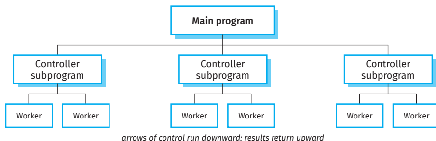
Figure 6.16 A main program/subprogram (call-and-return) architecture
