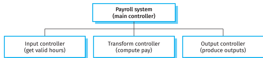
Figure 6.23 First-level factoring of the payroll system
