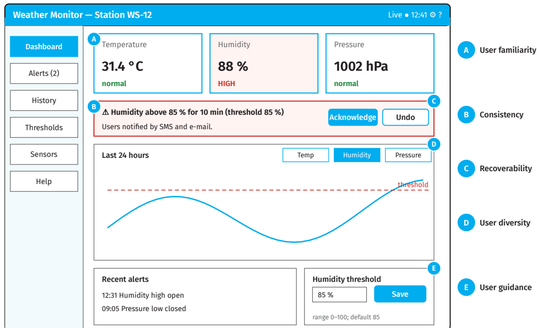
Figure 7.14 Annotated dashboard for the weather sensing and alert system
