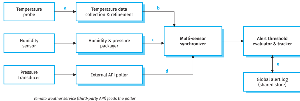
Figure 7.7 Module interactions in the weather sensing and alert system
