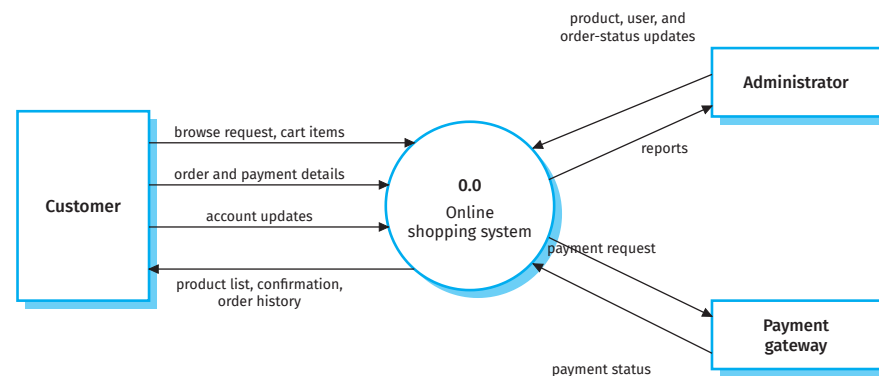
Figure 6.27 Context diagram of an online shopping system
