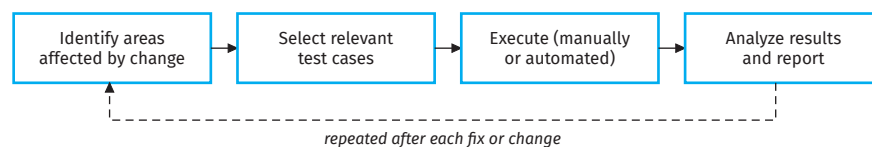
Figure 8.20 The regression testing cycle
