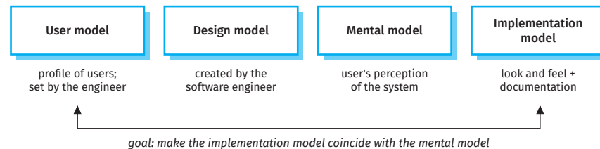
Figure 7.8 The four models of interface design
