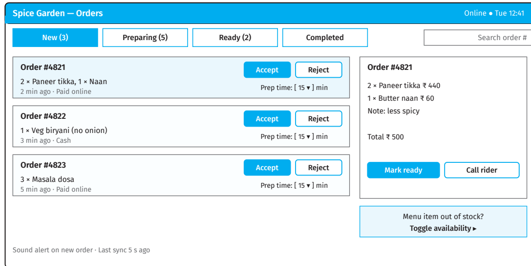
Figure 7.10 Layout of the restaurant order management screen
