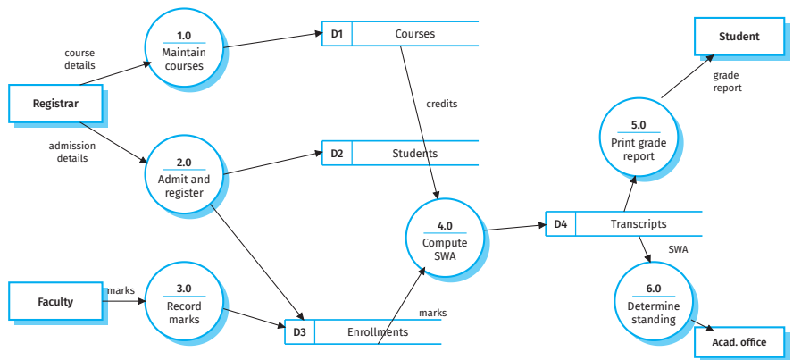
Figure 5.23 Level-1 DFD of the academic record system
