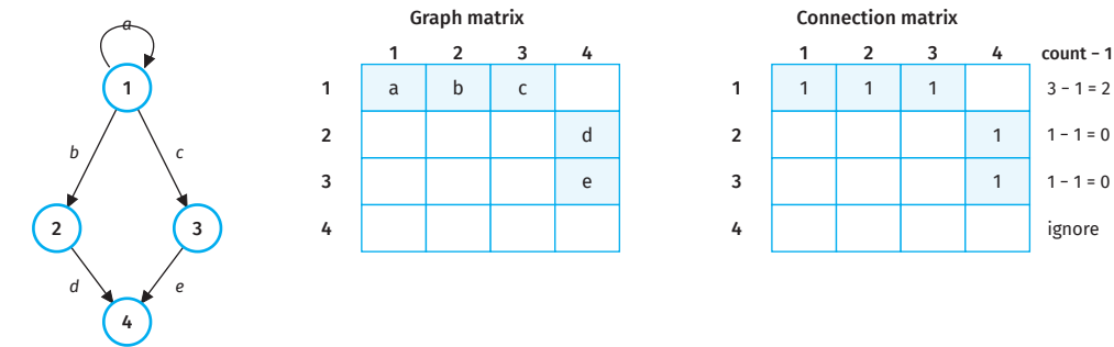
Figure 8.13 A flow graph with a self-loop, and its graph and connection matrices
