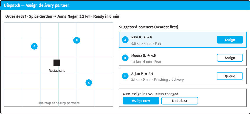
Figure 7.18 Layout of the delivery partner assignment screen
