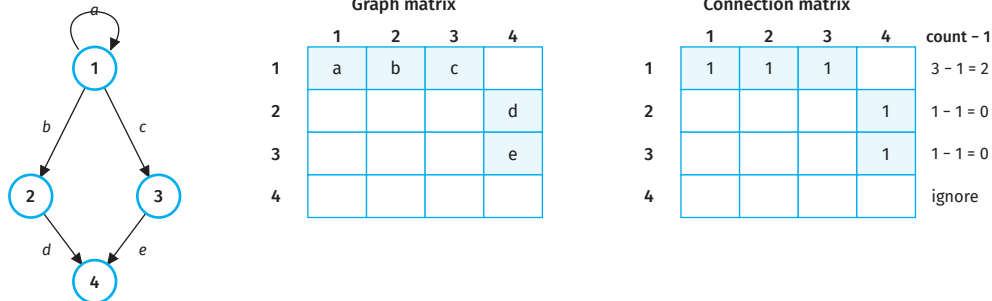
Figure 8.27 A flow graph with a self-loop, and its graph and connection matrices
