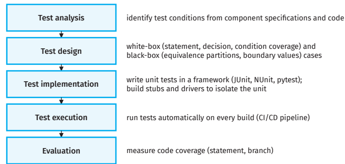
Figure 8.9 The component testing process
