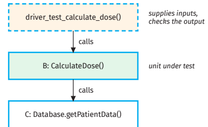
Testing B with a driver (A not yet developed)
