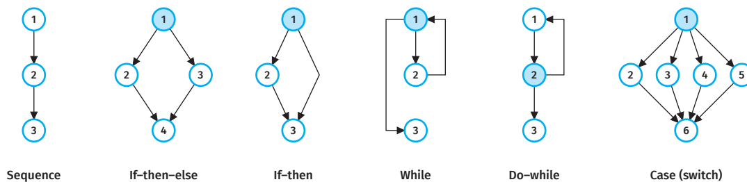
Figure 8.17 Flow-graph notation for structured constructs; shaded nodes are predicate nodes
