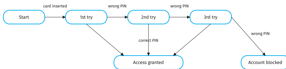
Figure 8.29 State transition diagram for PIN entry at an ATM
