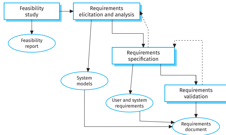
Figure 4.5 The requirements engineering process
