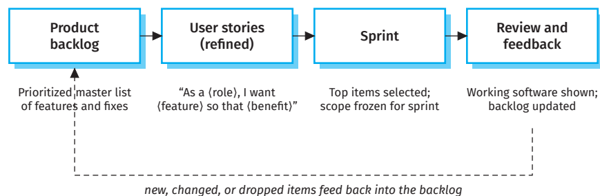
Figure 4.11 Requirements engineering in agile development
