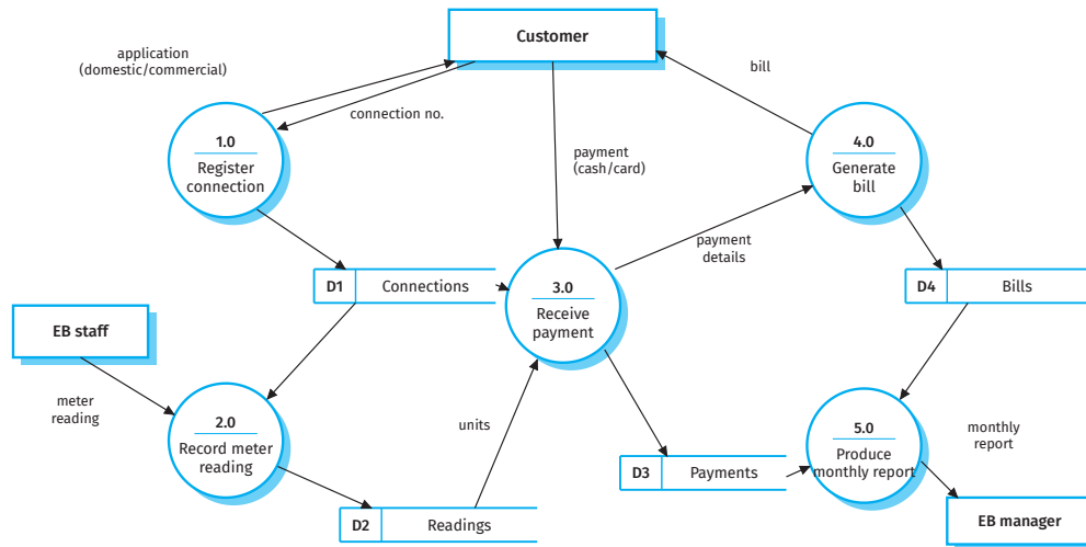
Figure 6.31 Level-1 DFD of the electricity billing system
