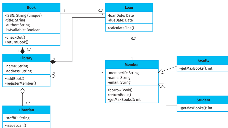
Figure 5.11 Class diagram of a library system
