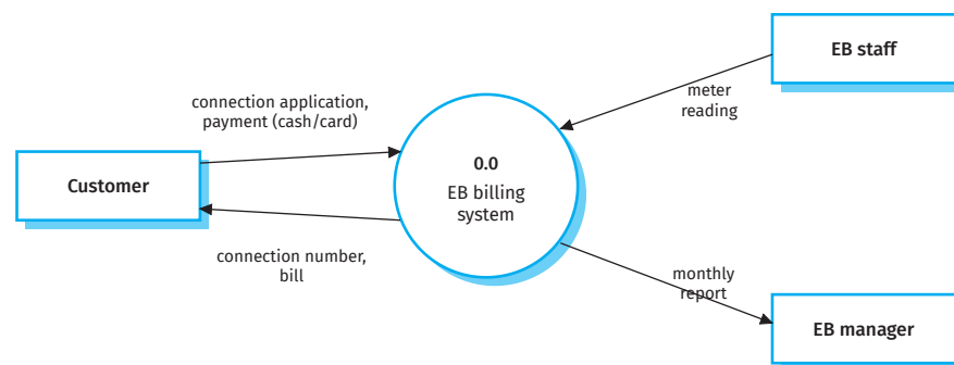
Figure 6.30 Context (level-0) diagram of the electricity billing system
