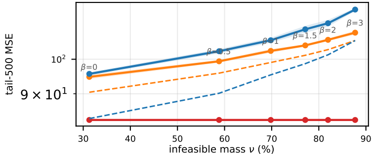
constant stepsize \eta
