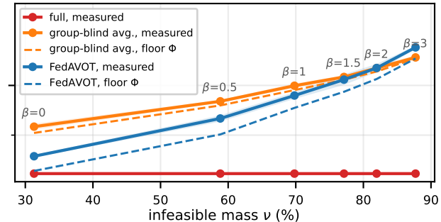
decaying stepsize \eta/(1 + t/1000)
