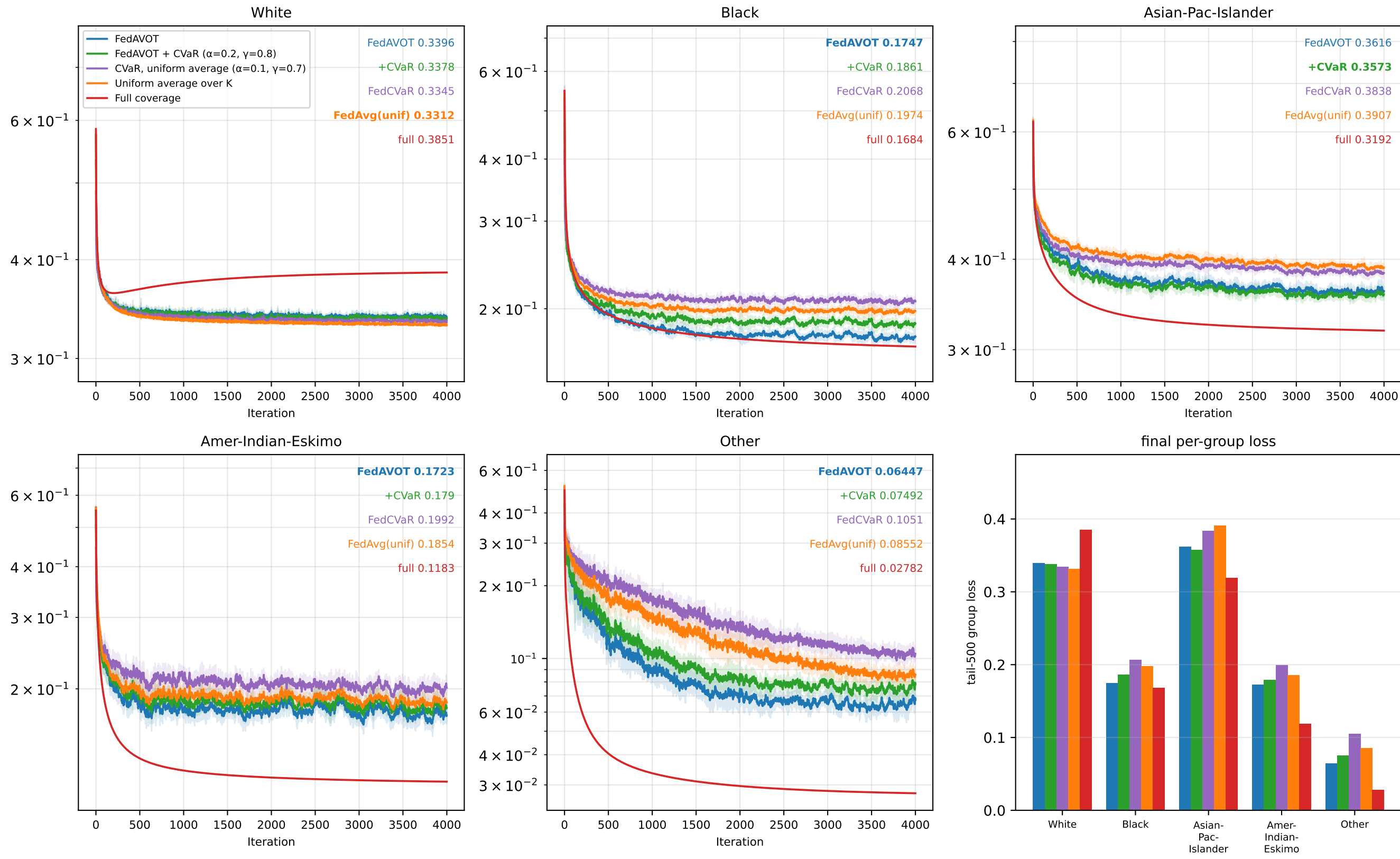
Adult income classification, INFEASIBLE regime: loss per critical group; (\alpha, \gamma) minimise the WORST-GROUP tail loss
