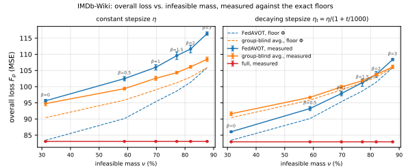
Figure 1: IMDb-Wiki severity sweep. Solid, measured tail-500 ( \pm 1 std); dashed, the exact floor \Phi(\cdot) each rule converges to. Left, constant stepsize: the optimization residual swamps the alignment gain and transport losses everywhere, even where the floors are seven units apart. Right, decaying stepsize: the residual collapses and the measured curves track their floors, so transport wins until the floors close at high \nu . The sign is set by which of the two terms of (9) dominates, not by the regime label.
