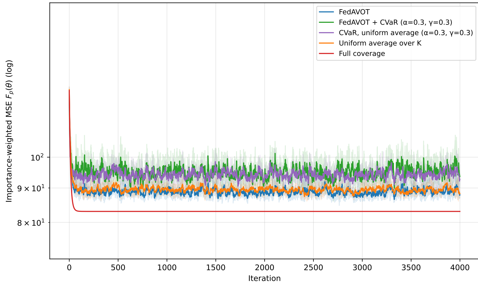
IMDb-Wiki age regression, FEASIBLE regime, 5 seeds tail overall: FedAVOT 89.08, +CVaR 95.51, FedCVaR 94.41, FedAvg(unif) 89.51, full 83.07
