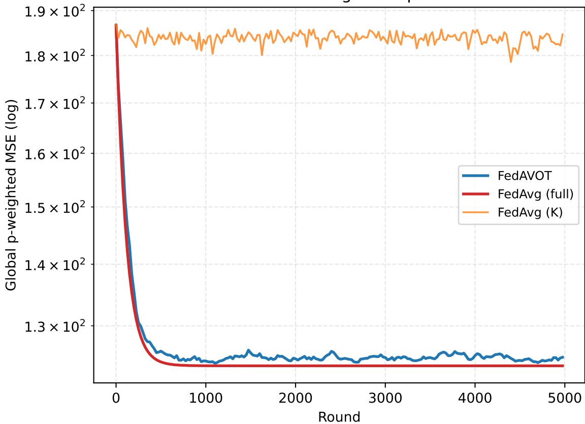
Feasible regime ( \alpha=0.5 , 14% infeasible), 5000 rounds FedAVOT converges to optimum
