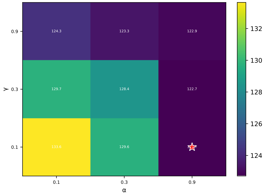
tail worst-group
