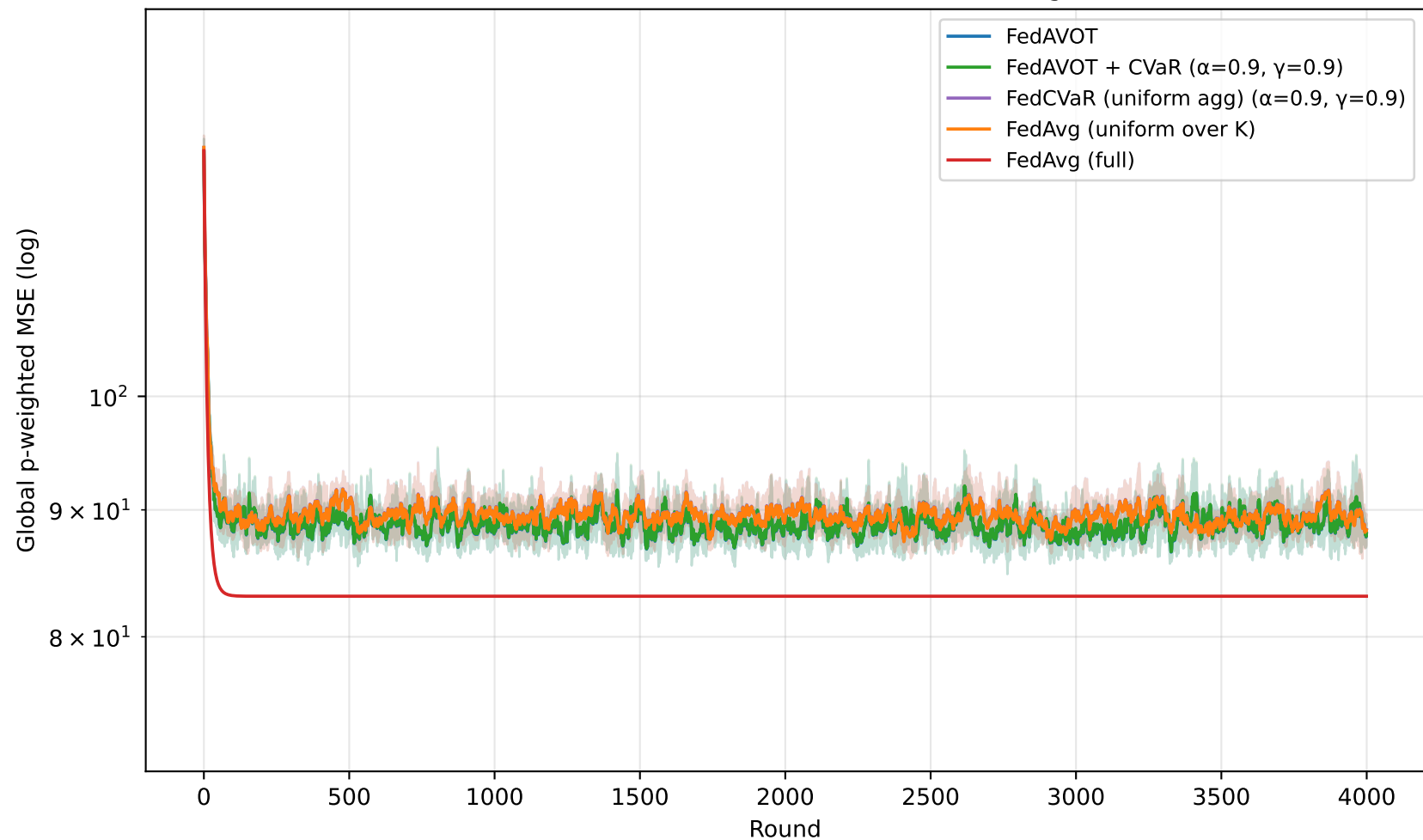
IMDb-Wiki age regression, FEASIBLE regime, 5 seeds tail overall: FedAVOT 89.08, +CVaR 89.15, FedCVaR 89.55, FedAvg(unif) 89.51, full 83.07
