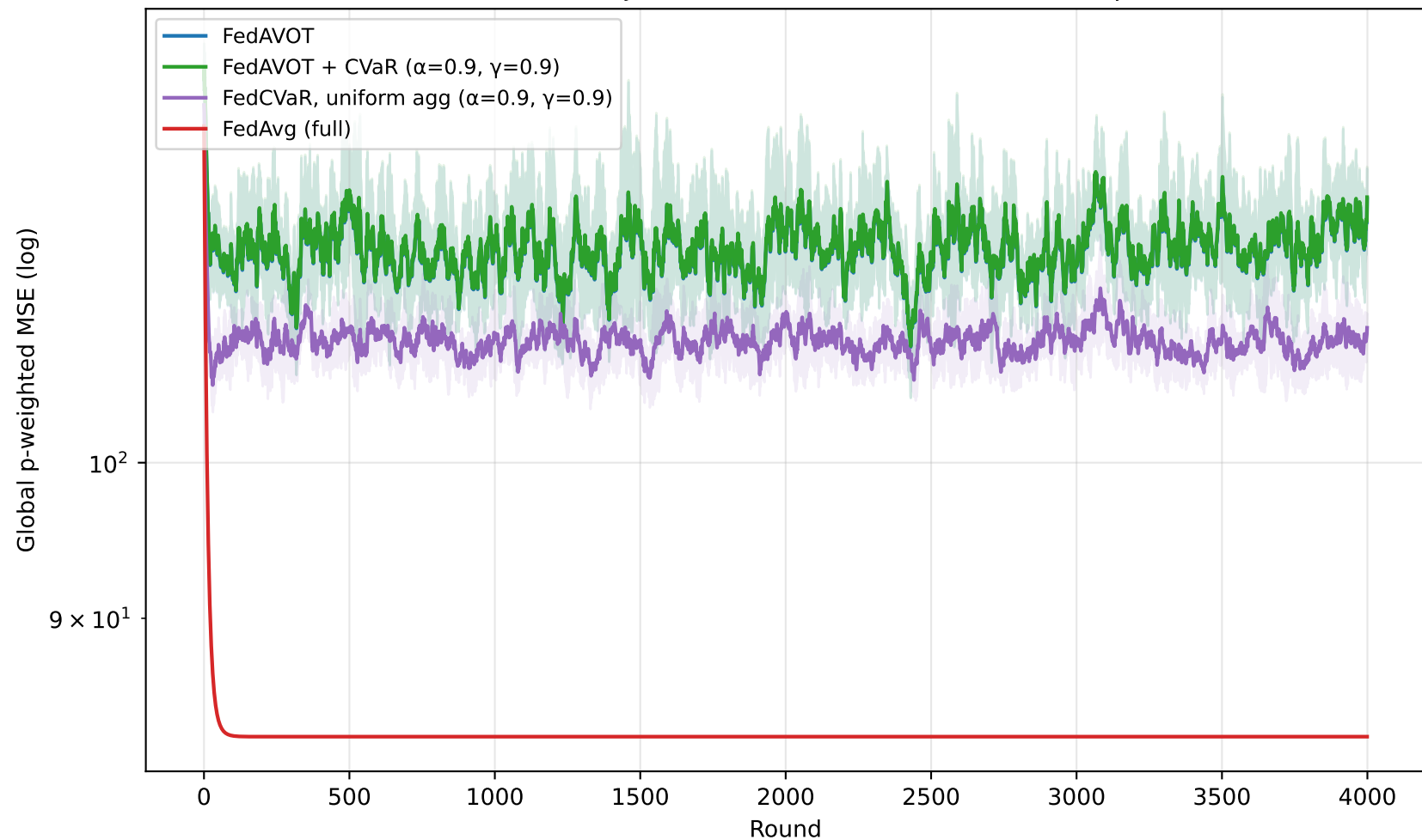
IMDb-Wiki, INFEASIBLE regime (mirrored cubic r), 4000 rounds, 5 seeds Does the CVaR risk-aware objective (arXiv:2309.14176) recover part of the floor?
