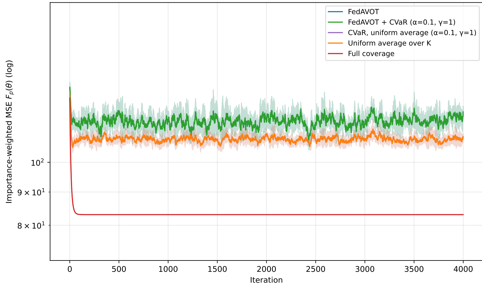
IMDb-Wiki age regression, INFEASIBLE regime, 5 seeds tail overall: FedAVOT 116.4, +CVaR 116.4, FedCVaR 108.5, FedAvg(unif) 108.5, full 83.07
