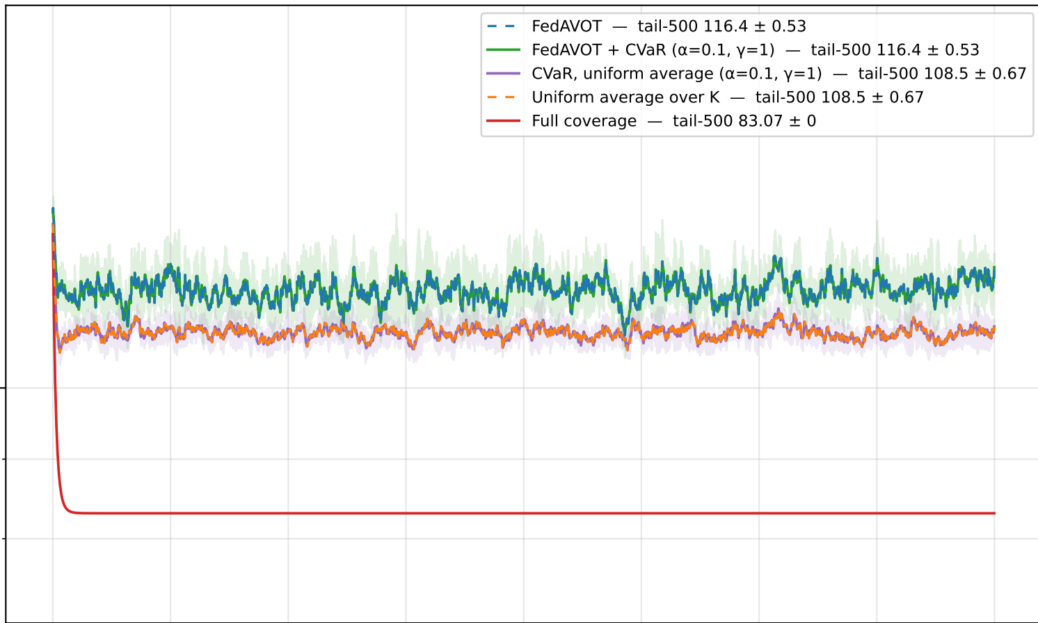
IMDb-Wiki age regression, INFEASIBLE regime, 5 seeds tail-500 = mean over the last 500 iterations, then mean \pm std across seeds
