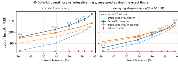
Figure 2: IMDB-Wiki severity sweep. Solid, measured tail-500 ( \pm 1 std); dashed, the exact floor \Phi(\cdot) each rule converges to. Left, constant stepsize: the optimization residual swamps the alignment gain and transport loses everywhere, even where the floors are seven units apart. Right, decaying stepsize: the residual collapses and the measured curves track their floors, so transport wins until the floors close at high \nu . The sign is set by which of the two terms of (9) dominates, not by the regime label.
