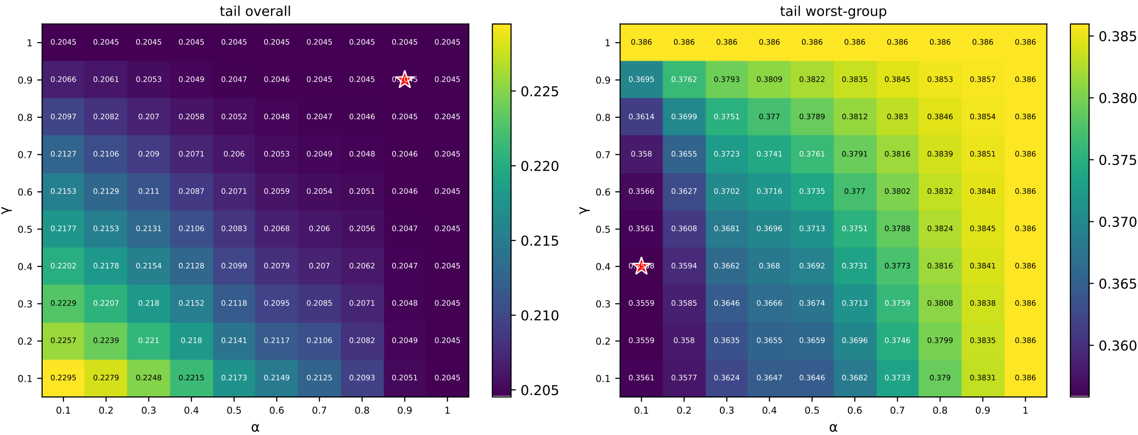
Adult income classification, FEASIBLE: FedAVOT + CVaR over (\alpha, \gamma) (mean over seeds; ★ = best incl. ties; \gamma=1 row and \alpha=1 column are exactly risk-neutral = FedAVOT)
