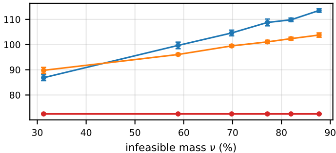
constant stepsize
