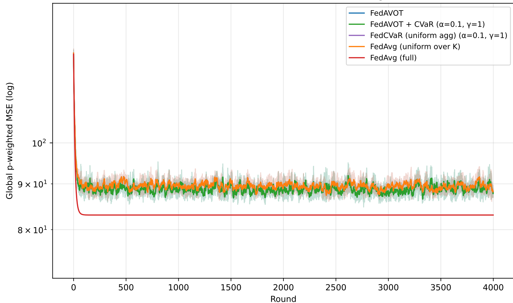
IMDb-Wiki age regression, FEASIBLE regime, 5 seeds tail overall: FedAVOT 89.08, +CVaR 89.08, FedCVaR 89.51, FedAvg(unif) 89.51, full 83.07
