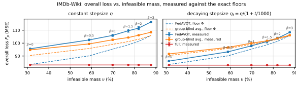
Figure 2: IMDb-Wiki severity sweep. Solid, measured tail-500 ( \pm 1 std); dashed, the exact floor \Phi(\cdot) each rule converges to. Left, constant stepsize: the optimization residual swamps the alignment gain and transport losses everywhere, even where the floors are seven units apart. Right, decaying stepsize: the residual collapses and the measured curves track their floors, so transport wins until the floors close at high \nu . The sign is set by which of the two terms of (9) dominates, not by the regime label.
