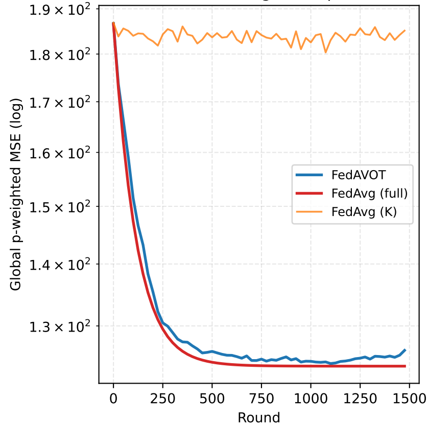
Feasible regime ( \alpha=0.5 , 14% infeasible)
