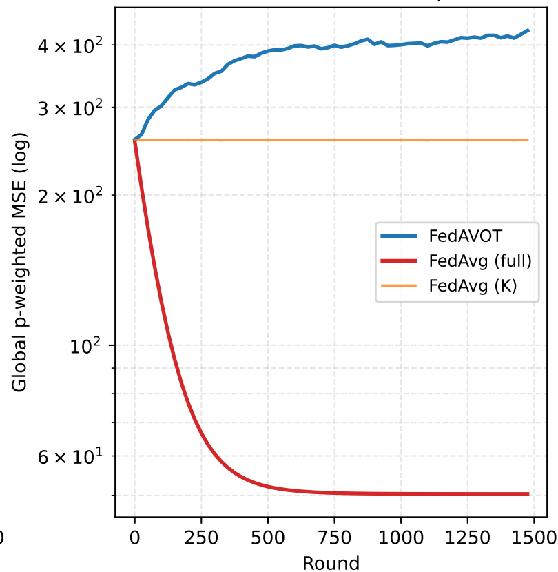
Infeasible regime ( \alpha=3.0 , 87% infeasible)
