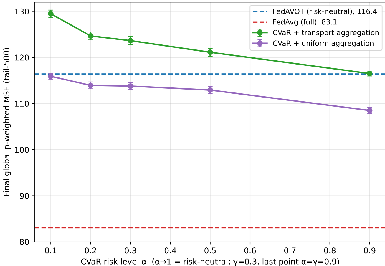
Infeasible IMDb-Wiki regime: turning CVaR OFF helps both schemes (more risk-aversion = worse; uniform averaging, not the hinge, is the win)
