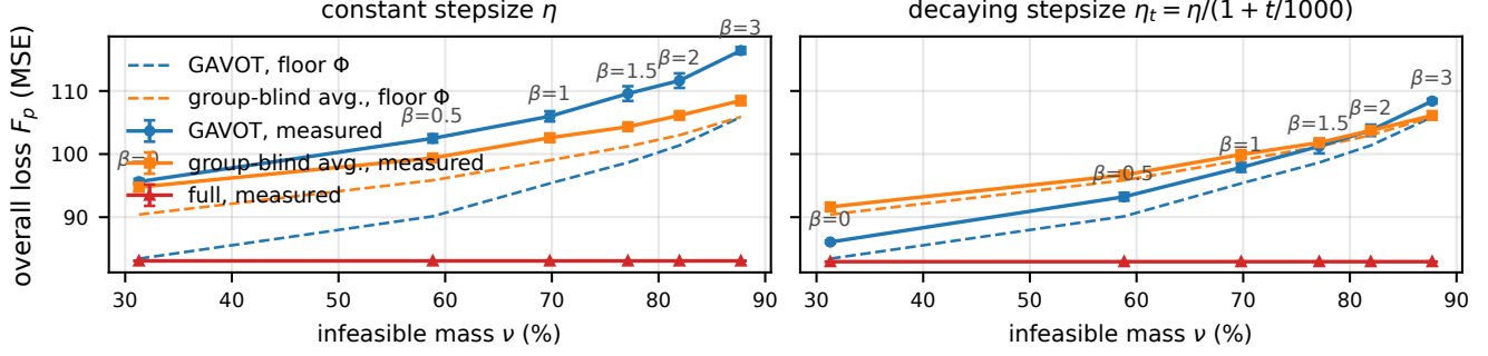
Fig. 2. IMDb-Wiki severity sweep: measured tail-500 (solid, \pm 1 std) against the exact floor \Phi(\cdot) of each rule (dashed). Left, constant stepsize: the residual swamps the alignment gain and transport losses everywhere. Right, decaying: the curves track their floors and transport wins until the floors close at high \nu .
