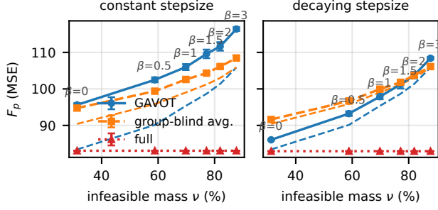
Fig. 2. IMDb-Wiki severity sweep: measured tail-500 (solid, \pm 1 std) against the exact floor \Phi(\cdot) of each rule (dashed). Left, constant stepsize: the residual swamps the alignment gain and transport loses everywhere. Right, decaying: the curves track their floors and transport wins until the floors close at high \nu .
