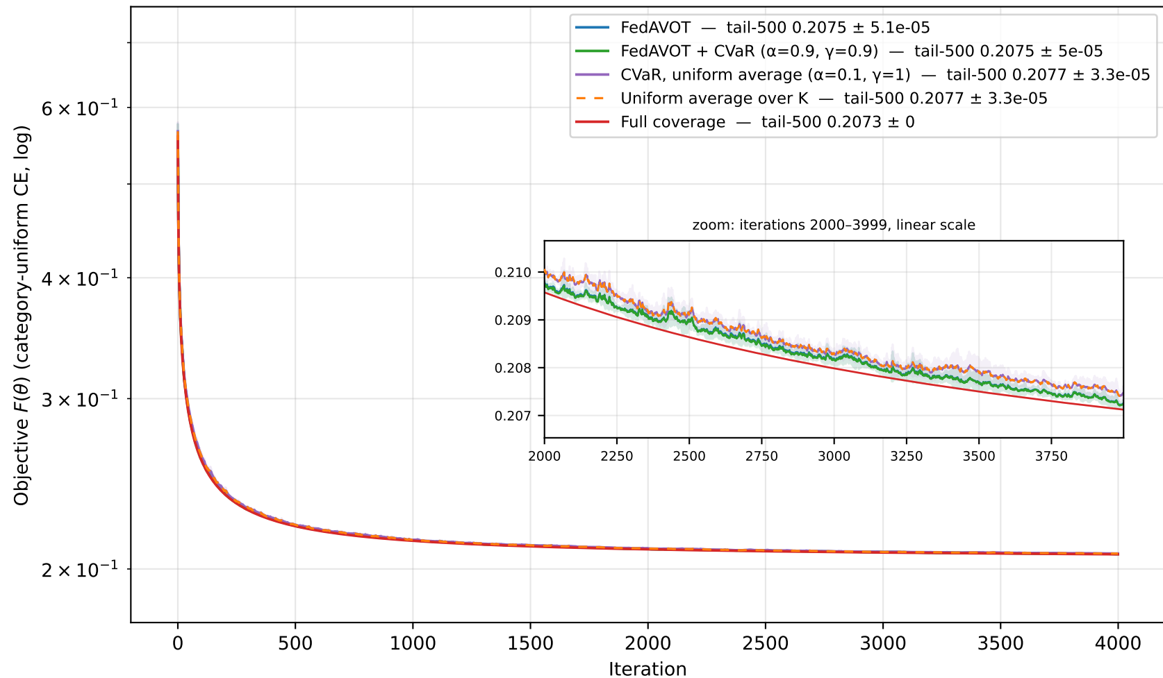
Adult income classification, FEASIBLE regime, 5 seeds tail-500 = mean over the last 500 iterations, then mean \pm std across seeds
