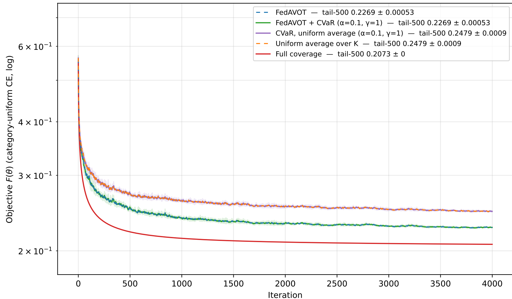
Adult income classification, INFEASIBLE regime, 5 seeds tail-500 = mean over the last 500 iterations, then mean \pm std across seeds
