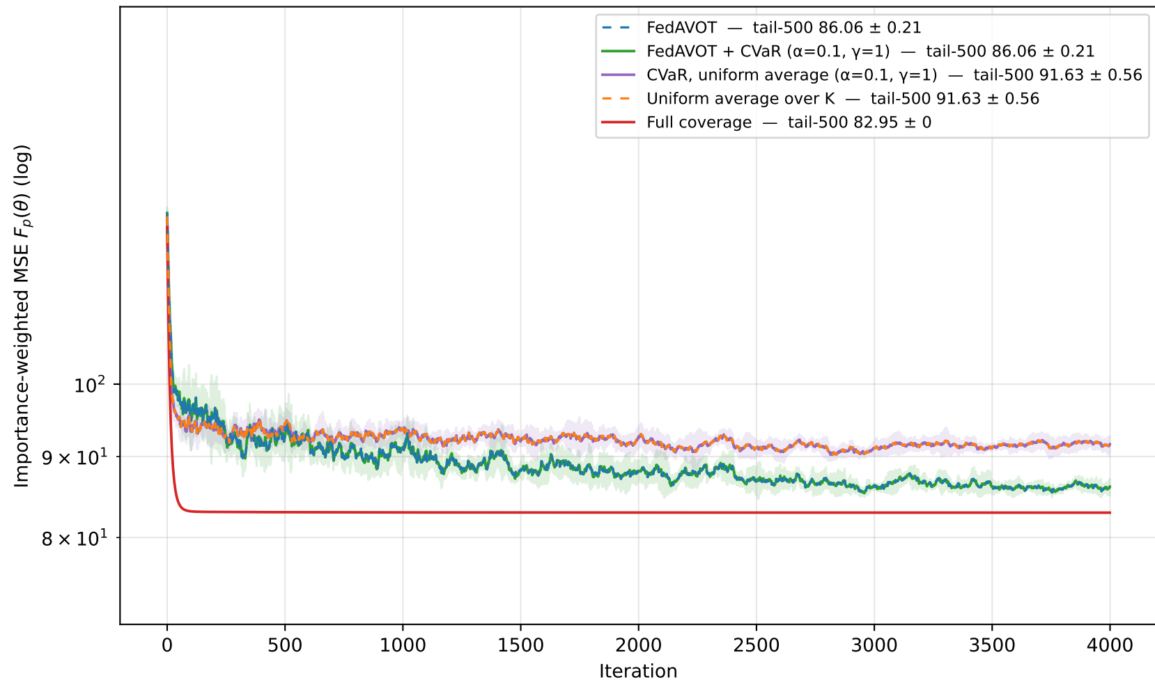
IMDb-Wiki age regression, INFEASIBLE regime, 5 seeds tail-500 = mean over the last 500 iterations, then mean \pm std across seeds
