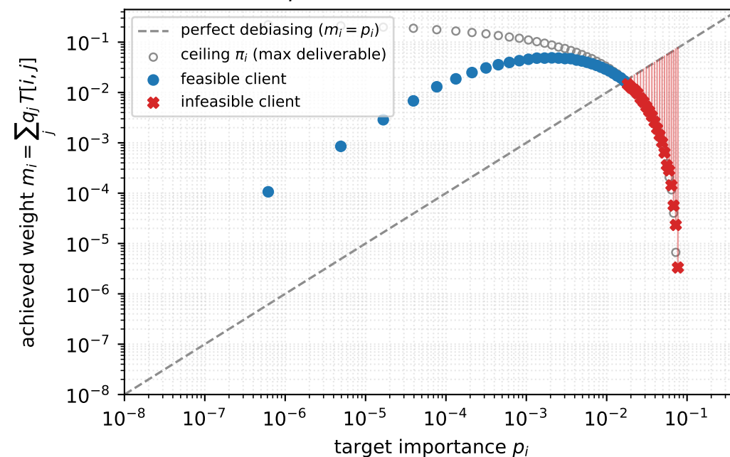
Infeasible ( \alpha=3.0 ): high- p clients pinned at ceiling 78% of p -mass undelivered \Rightarrow loss floor
