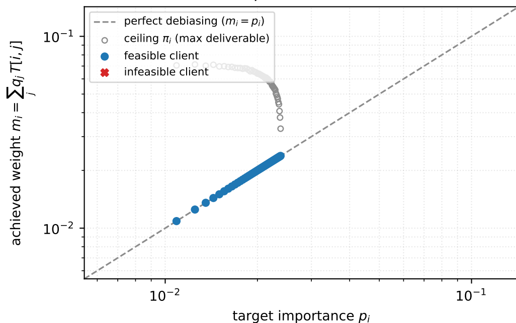
Feasible ( \alpha=0.2 ): IPFP hits the target 0.0% of p -mass undelivered
