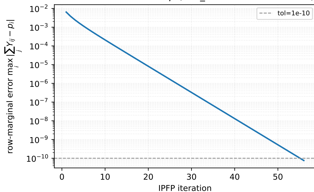
Feasible: IPFP matches p (row_err \rightarrow 8e-11 in 56 iters)
