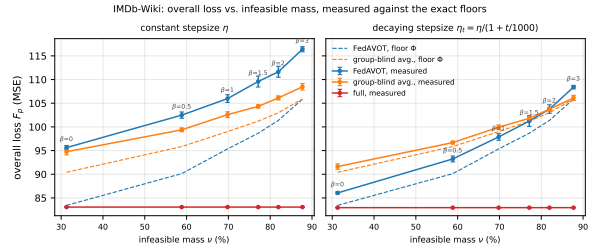
Figure 1: IMDb-Wiki severity sweep. Solid, measured tail-500 ( \pm 1 std); dashed, the exact floor \Phi(\cdot) each rule converges to. Left, constant stepsize: the optimization residual swamps the alignment gain and transport losses everywhere, even where the floors are seven units apart. Right, decaying stepsize: the residual collapses and the measured curves track their floors, so transport wins until the floors close at high \nu . The sign is set by which of the two terms of (9) dominates, not by the regime label.
