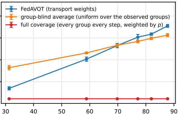
decaying stepsize \eta_t = \eta/(1 + t/1000)
