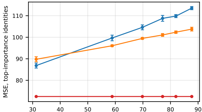
constant stepsize \eta
