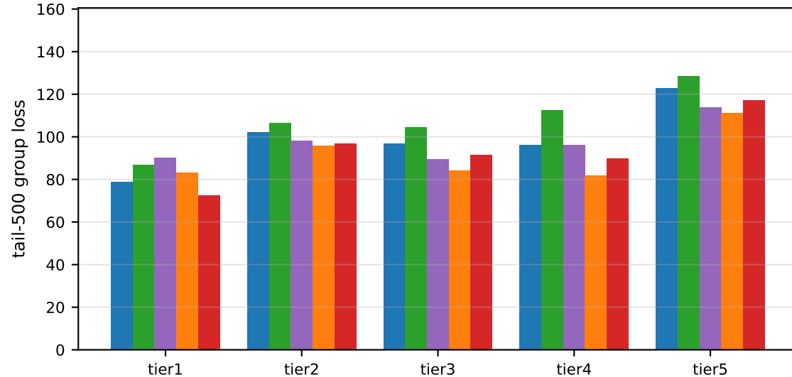
Adult, FEASIBLE
