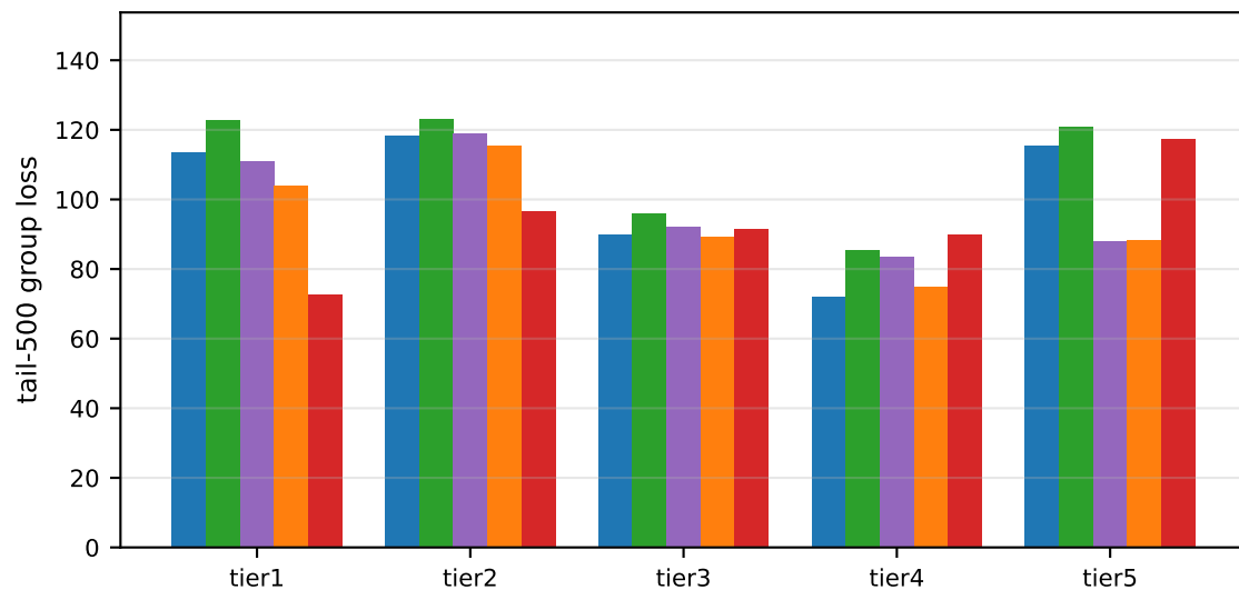
Adult, INFEASIBLE
