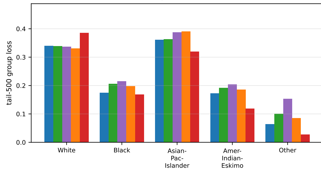
Adult, INFEASIBLE
