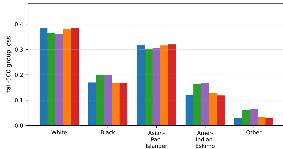
Adult, FEASIBLE
