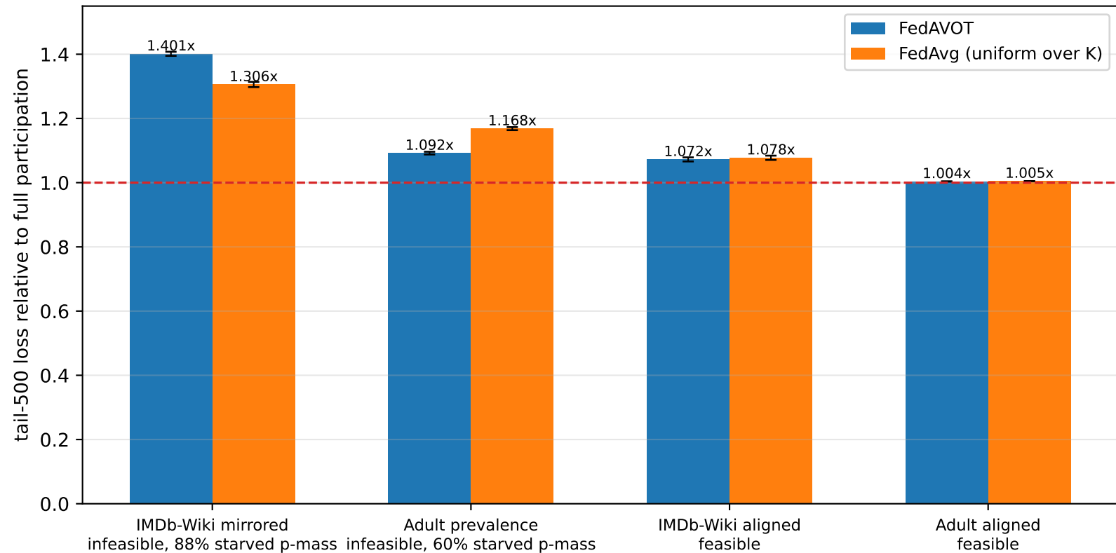
Uniform averaging wins only under severe infeasibility (tail-500 mean over 5 seeds, each model at its best config)
