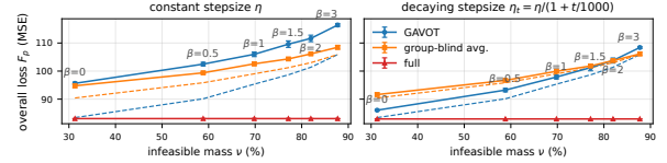
Fig. 2. IMDb-Wiki severity sweep. Solid, measured tail-500 ( \pm 1 std); dashed, the exact floor \Phi(\cdot) each rule converges to. Left, constant stepsize: the optimization residual swamps the alignment gain and transport loses everywhere, even where the floors are seven units apart. Right, decaying stepsize: the residual collapses and the measured curves track their floors, so transport wins until the floors close at high \nu . The sign is set by which of the two terms of (9) dominates, not by the regime label.
