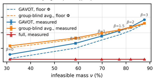
decaying stepsize \eta_t = \eta/(1 + t/1000)
