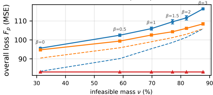
constant stepsize \eta
