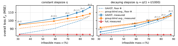
Fig. 1. IMDb-Wiki severity sweep. Solid, measured tail-500 ( \pm 1 std); dashed, the exact floor \Phi(\cdot) each rule converges to. Left, constant stepsize: the optimization residual swamps the alignment gain and transport loses everywhere, even where the floors are seven units apart. Right, decaying stepsize: the residual collapses and the measured curves track their floors, so transport wins until the floors close at high \nu . The sign is set by which of the two terms of (9) dominates, not by the regime label.
