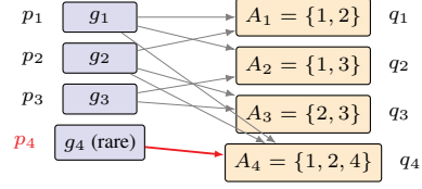
Fig. 1. The mask E : compositions carry the mass q they occur with, groups must receive the mass p the objective assigns. Group 4 is reachable only through A_4 , so alignment needs p_4 \leq q_4 , the Hall condition of Thm. 3 on I = \{4\} ; a smaller batch deletes A_4 and makes p_4 unreachable.
