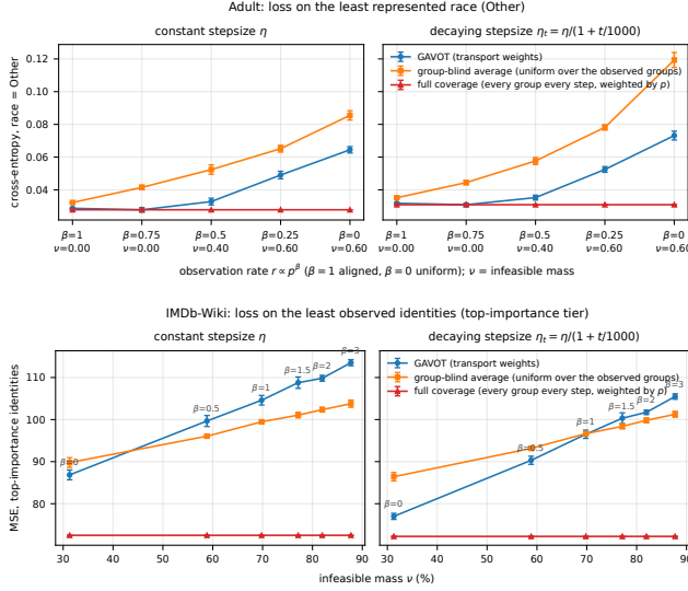
Fig. 3. Loss on the least represented group, the metric the fairness target is about. Top, Adult: cross-entropy on race Other, one group of 30 out of 100, to which the category-uniform target assigns p_i = 0.2 ; the axis is the observation-rate exponent, \beta=1 aligned, \beta=0 uniform (prevalence). Bottom, IMDB-Wiki: MSE on the 20 highest-importance identities, the least observed ones once \beta > 0 , against \nu . Left panels constant stepsize, right panels decaying. Same protocol as the tables ( K=3 , H=5 , 4000 steps, tail-500 mean \pm std over 5 seeds); lower is better. Curves are the group-wise entries of the same runs as Table 1 and Fig. 2.
