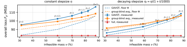
Fig. 2. IMDb-Wiki severity sweep. Solid, measured tail-500 ( \pm 1 std); dashed, the exact floor \Phi(\cdot) each rule converges to. Left, constant stepsize: the optimization residual swamps the alignment gain and transport loses everywhere, even where the floors are seven units apart. Right, decaying stepsize: the residual collapses and the measured curves track their floors, so transport wins until the floors close at high \nu . The sign is set by which of the two terms of (9) dominates, not by the regime label.
