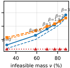
decaying stepsize
