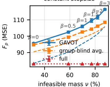
constant stepsize
