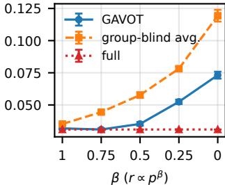
Adult: race Other (CE)
